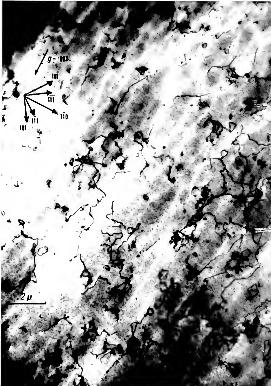
Figure 49.--Electron micrograph of a foil containing large prismatic loops and heavily jogged dislocation lines. Note the preponderance of line segments lying along projected \langle 110 \rangle and \langle 112 \rangle directions.
